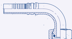
Interlock 90° Swept Female Metric Heavy Serie 24° Cone Seat Swivel (DKOS 90)
