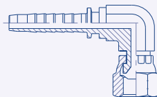
90° Swept Compact Female BSP Parallel Pipe Swivel 23.3082
