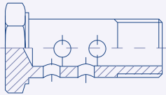
Metric Banjo Double Bolt 88.1652
