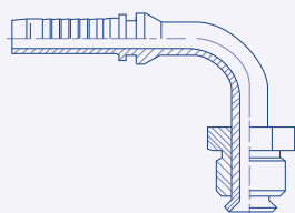
SAE Inverted 45° Flare 90° Elbow Male 23.2290
