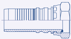
Interlock Female BSP Parallel Pipe with O-ring Swivel (DKOR) 26.3112
