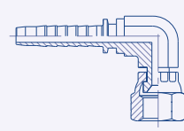
90° Compact Female JIC 37° Swivel 23.4082
