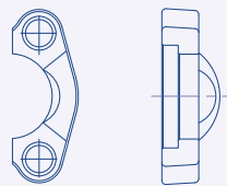
Split Flange 6000 PSI (code 62) 88.5600
