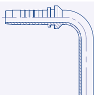
90° Swept Metric Standpipe (BEL 90) 23.6090
