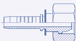
Female Metric 24°/60° Cone Seat Swivel (DKL) 23.5213
