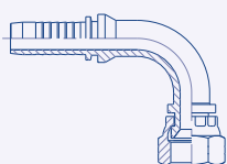
90° Swept Female SAE 45° Swivel 23.4S92
