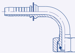
90° Swept Female Metric French Serie 24° Cone Seat Swivel (DKF) 23.5593
