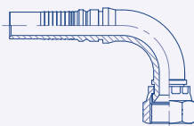
Interlock 90° Swept Female JIC 37° Swivel (DKJ 90°) 26.4092
