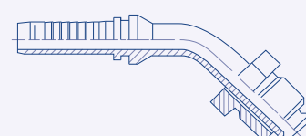
SAE Inverted 45° Flare 45° Elbow Male 23.2240
