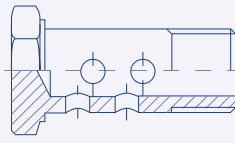
BSP Banjo Double Bolt 88.1602
