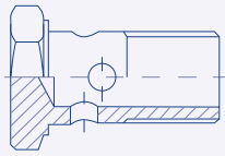
BSP Banjo Bolt 88.1600
