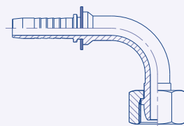
90° Swept Female Metric 24°/60° Cone Seat Swivel (DKL) 23.5293
