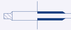
Metric Bonded Seals 88.2004
